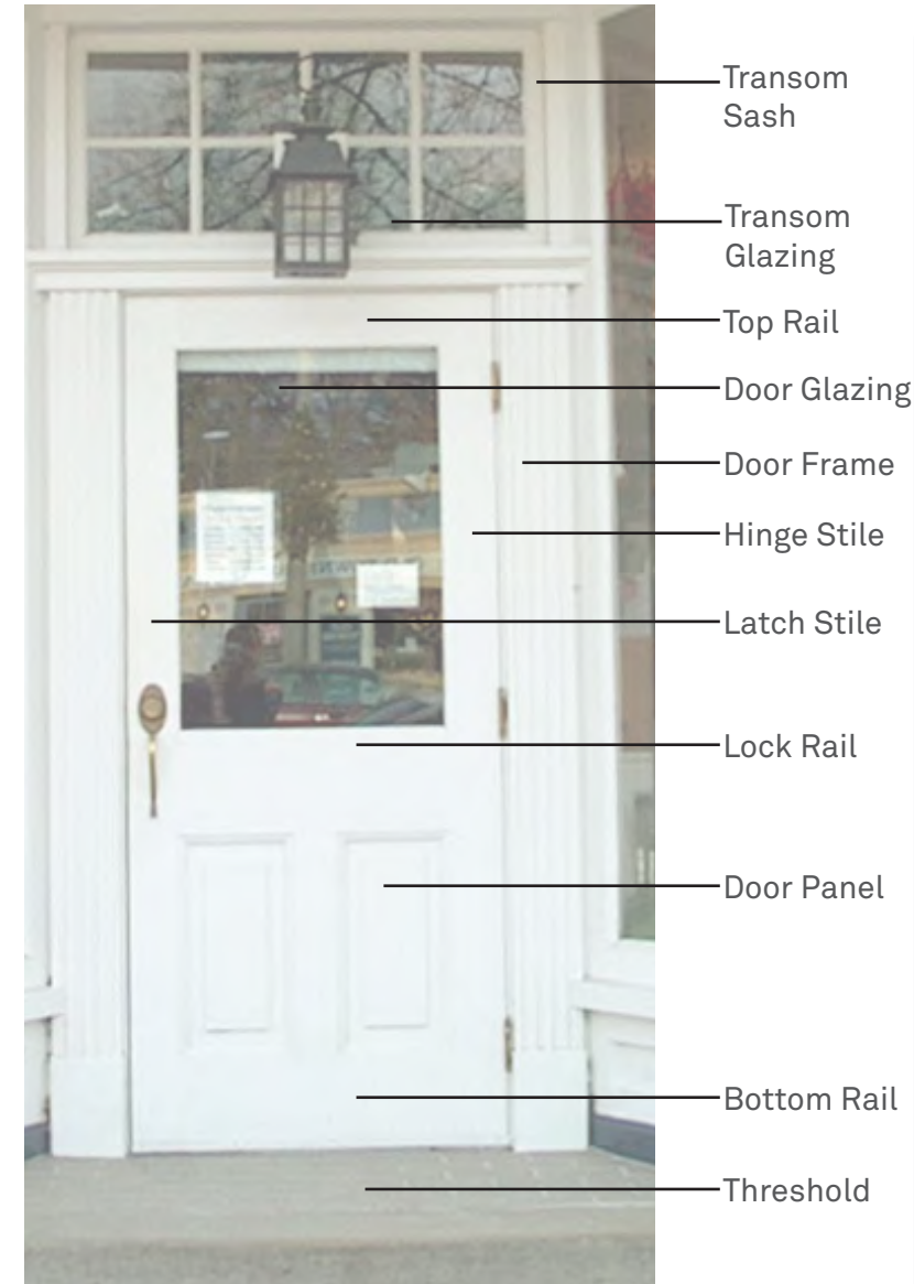
Figure 17 Typical heritage door details
